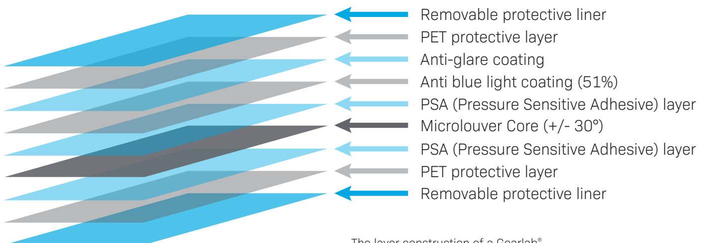
The layer construction of a Gearlab® Privacy Filter: Black Glossy/Black Matte.
